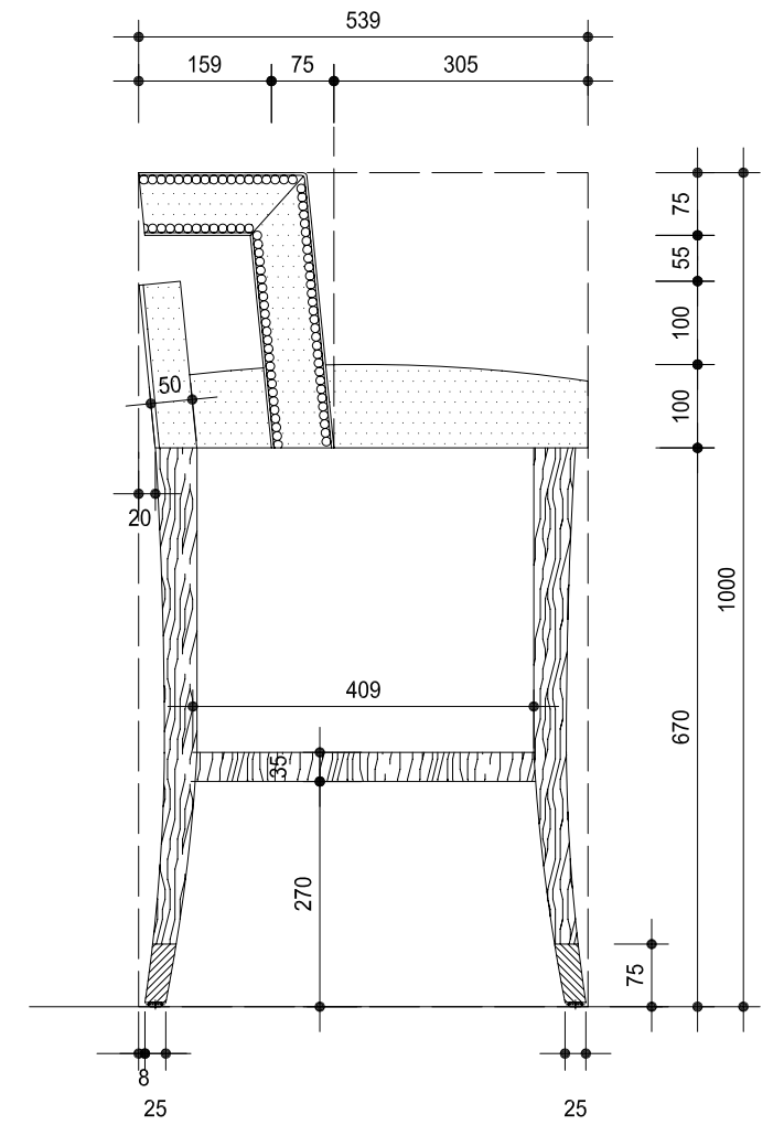
REAR ELEVATION
