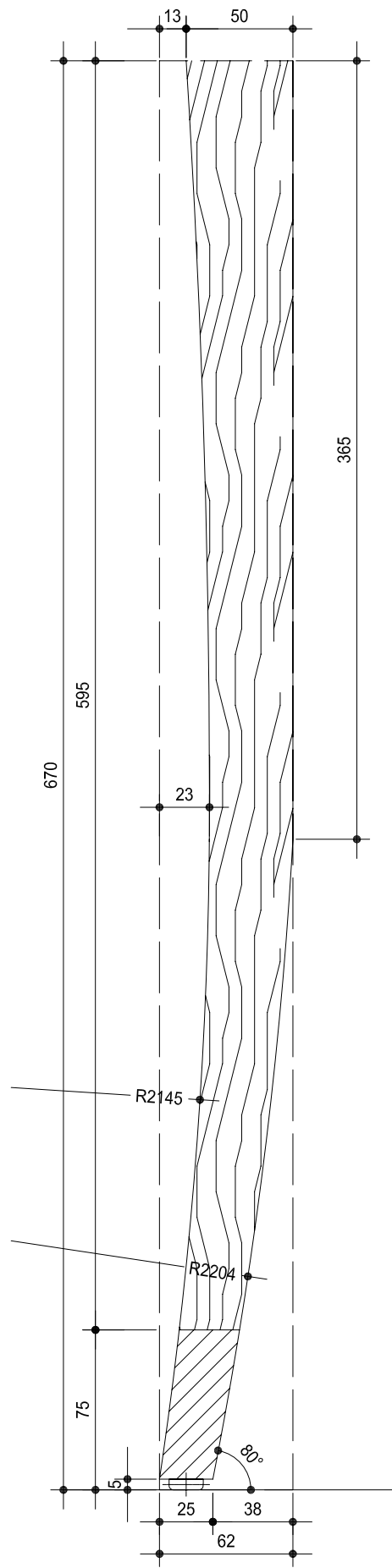
LEG DETAIL
