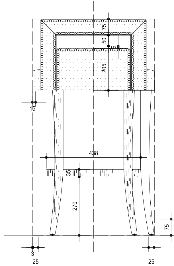
REAR ELEVATION
