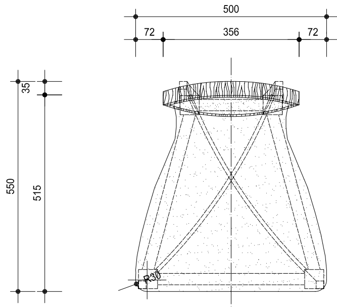
BAR STOOL PLAN
