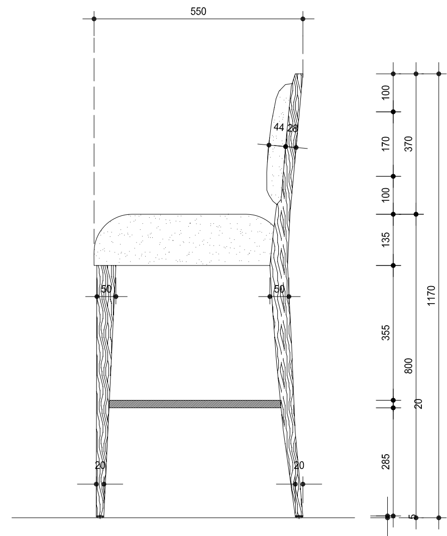
SIDE ELEVATION
