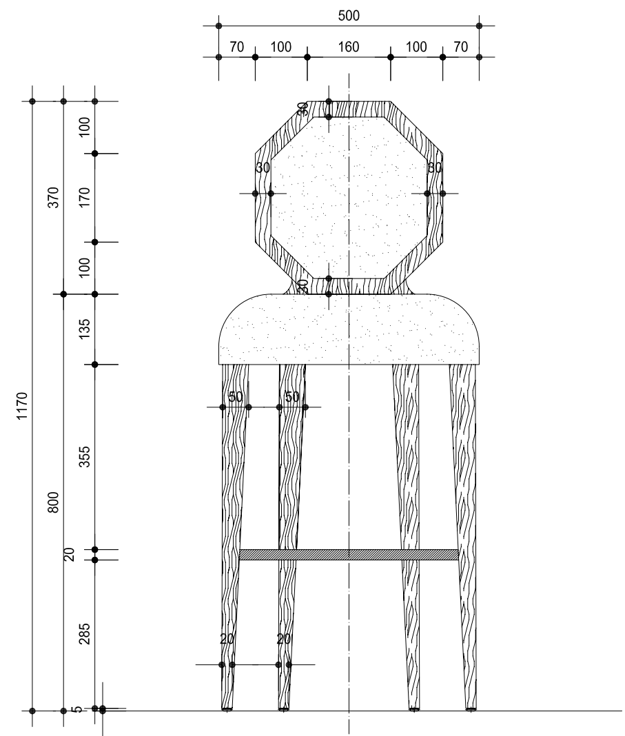
FRONT ELEVATION
