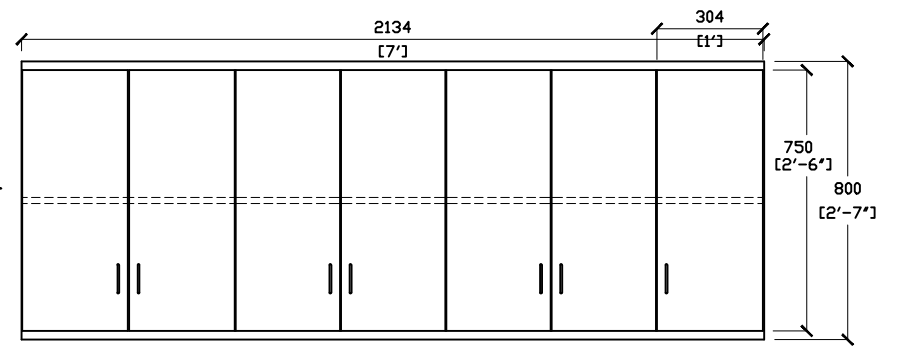
CUPBOARD TWO (2) FRONT VIEW
