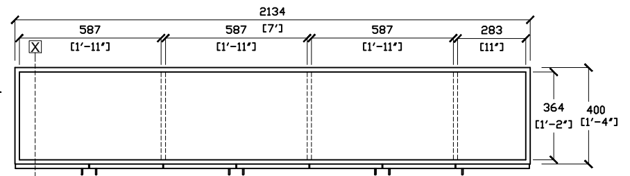
CUPBOARD TWO (2) TOP VIEW
