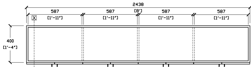
CUPBOARD ONE (1) TOP VIEW
