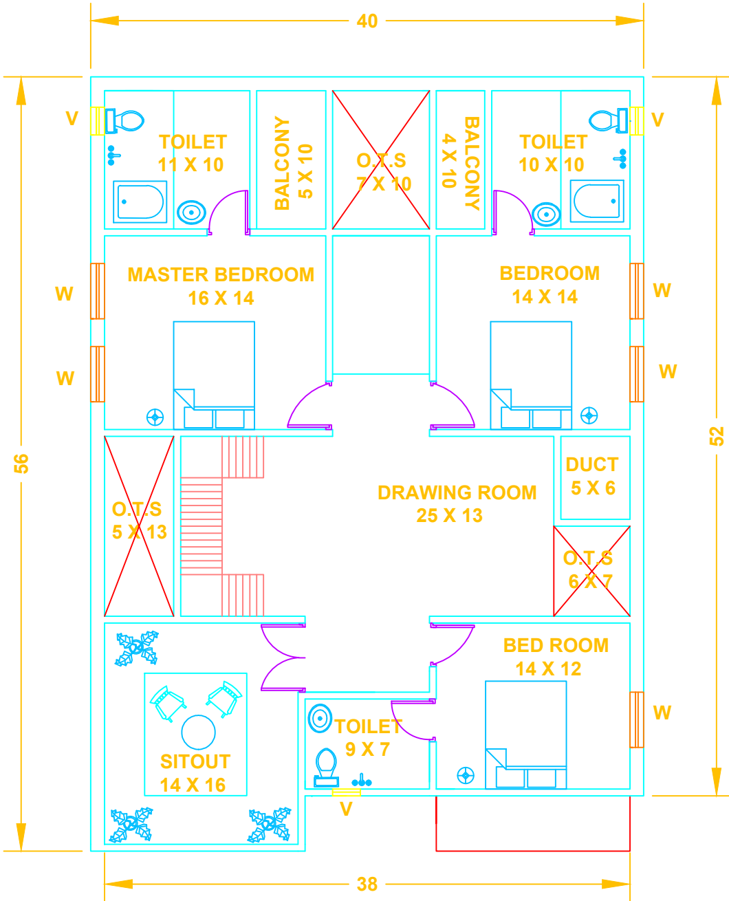
FIRST FLOOR
