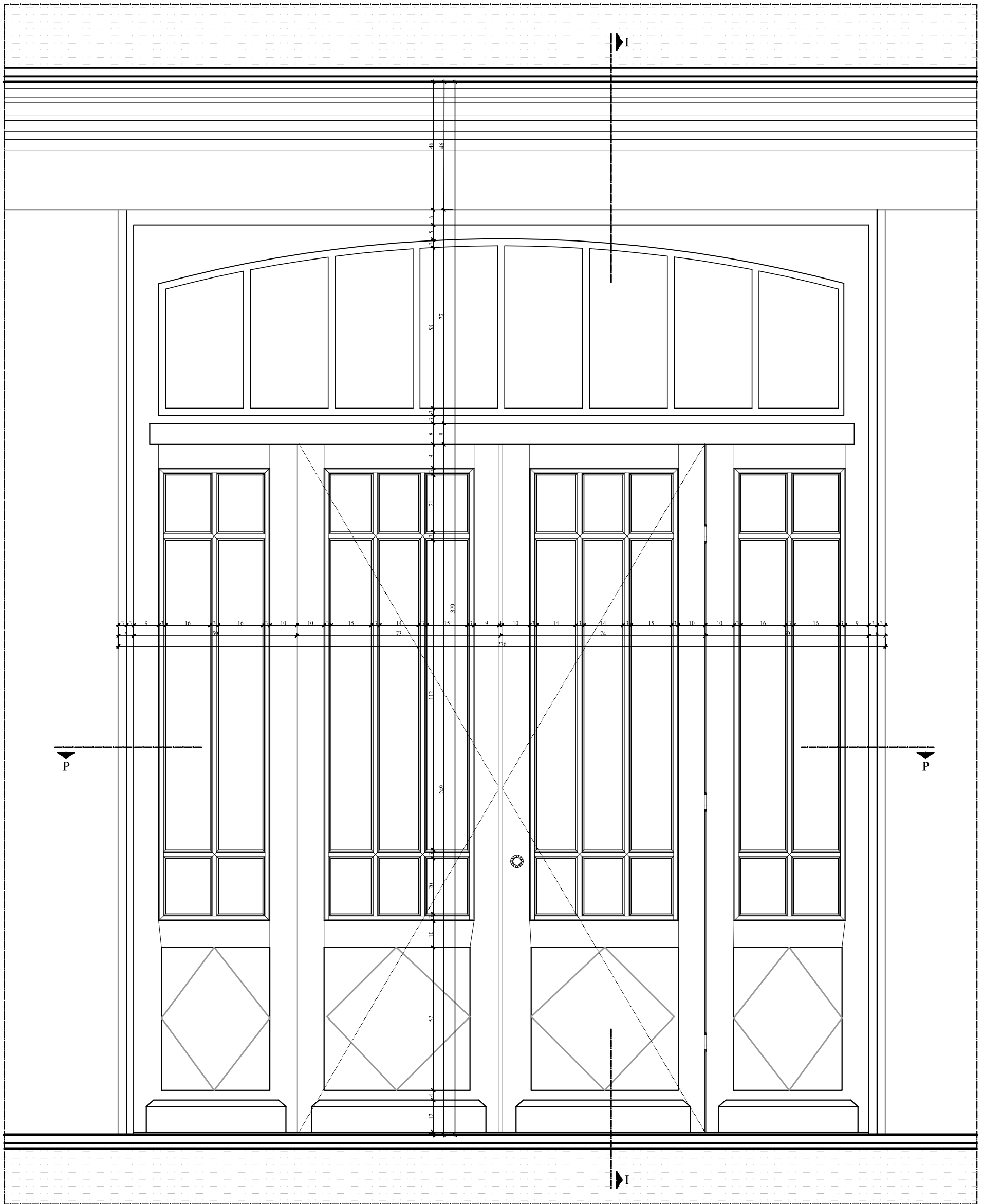
EXTERIOR ELEVATION
