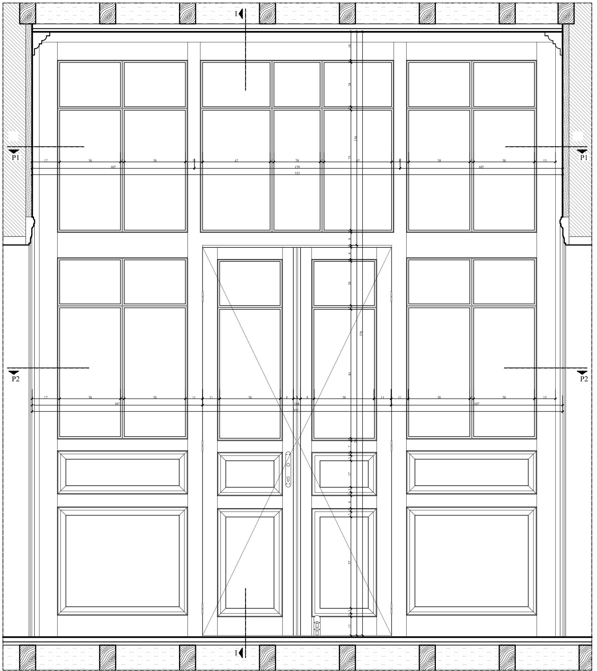
EXTERIOR ELEVATION
