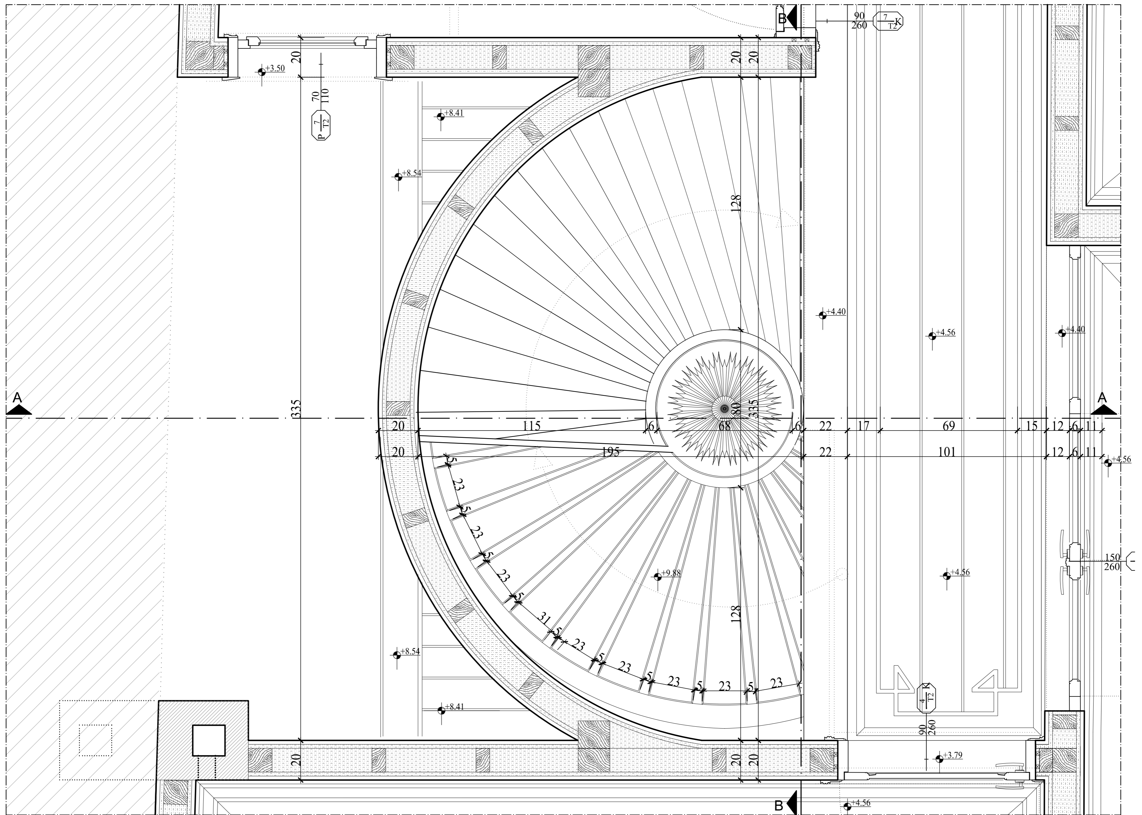
GROUND FLOOR CEILING PLAN SCALE : 1/20
