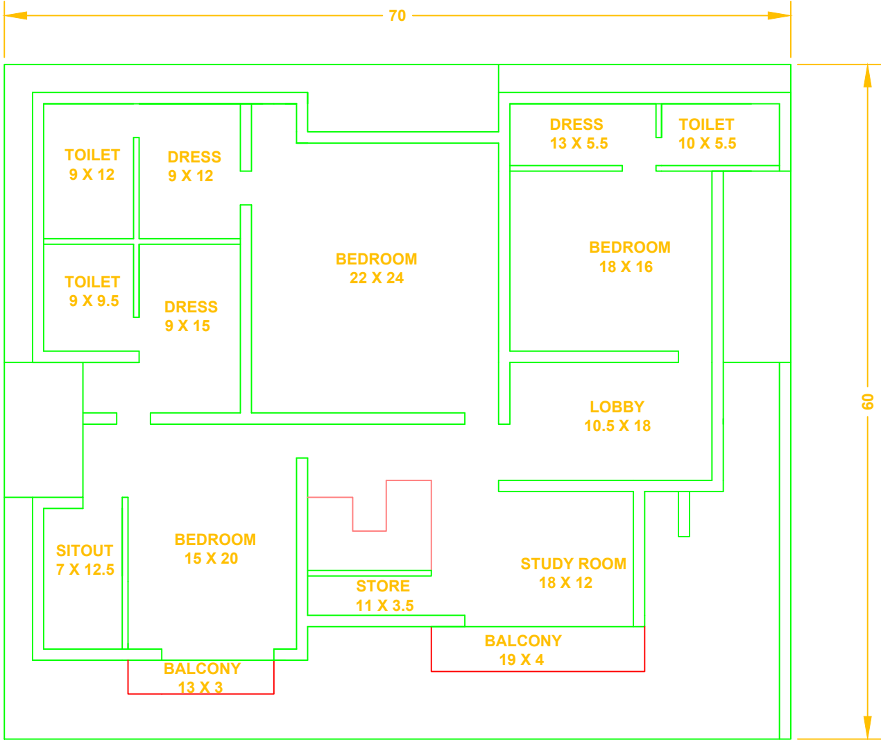
FIRST FLOOR
