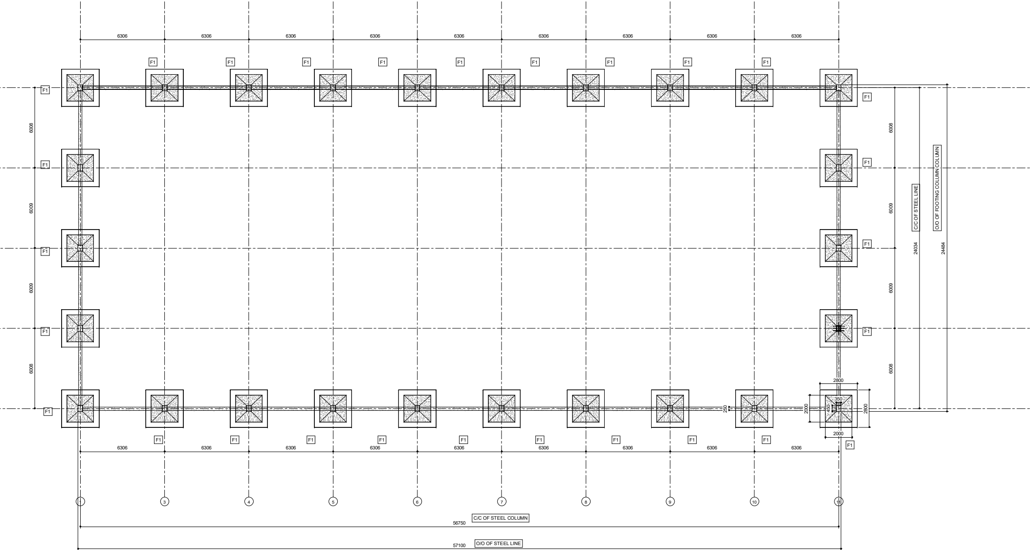
LAYOUT PLAN
