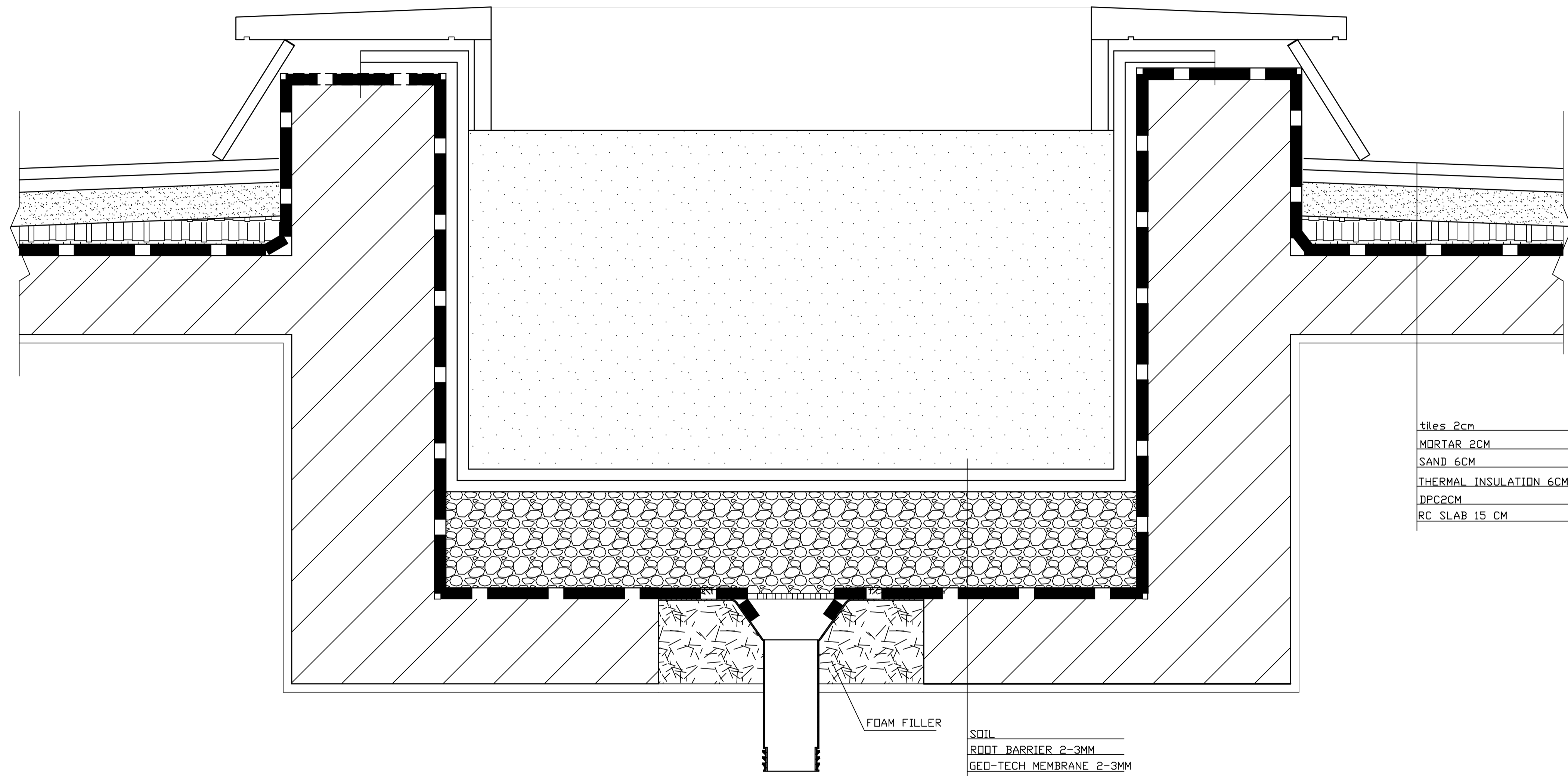
1 PLANTER DETAIL SCALE 1:5
