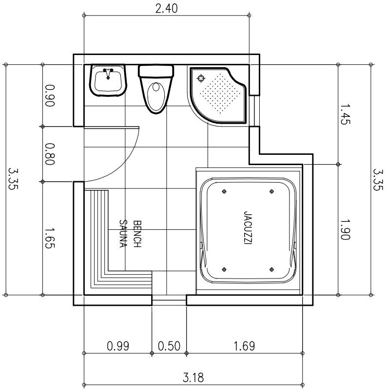
1 A-1 MASTER'S T&B OPTION 1 PROPOSED FLOOR PLAN SCALE : 1:50 MTS.
