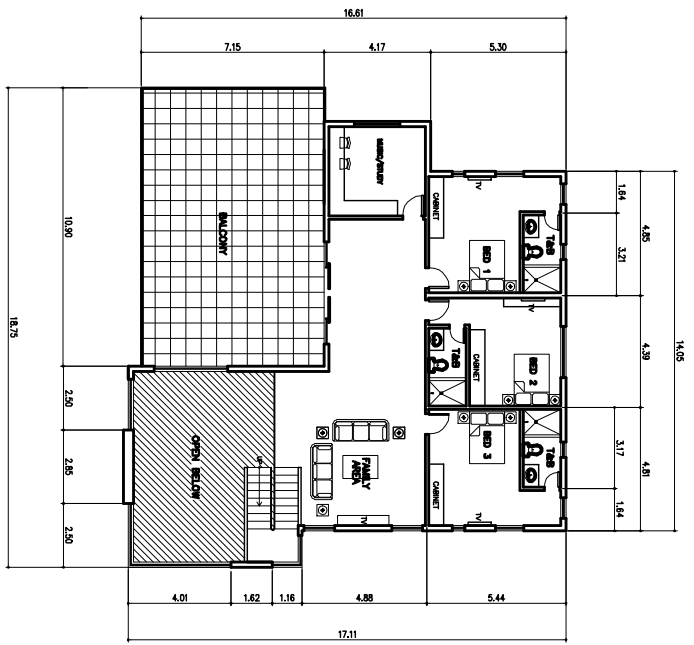
B A-2 278 SQUARES PROPOSED SECOND FLOOR SCALE: 1:100 U.S.
