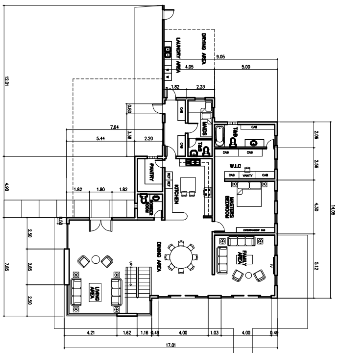
A A-2 210 SQUARES PROPOSED GROUND FLOOR SCALE: 1:100 U.S.
