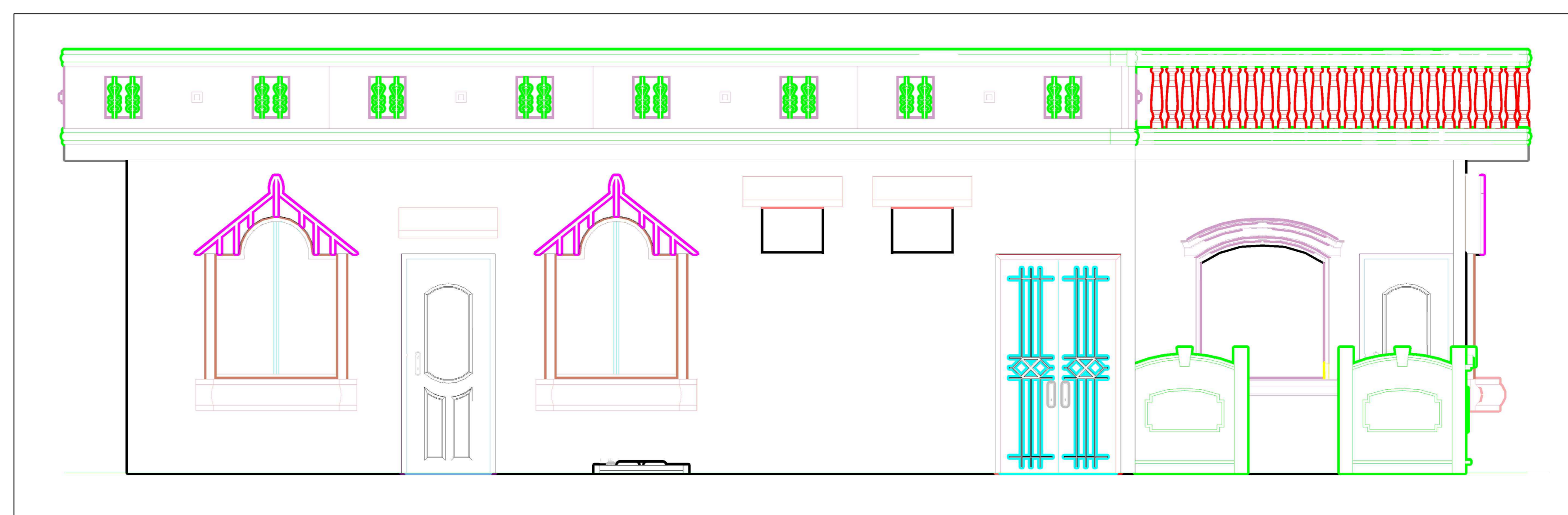
FRONT ELEVATION DEATIL
