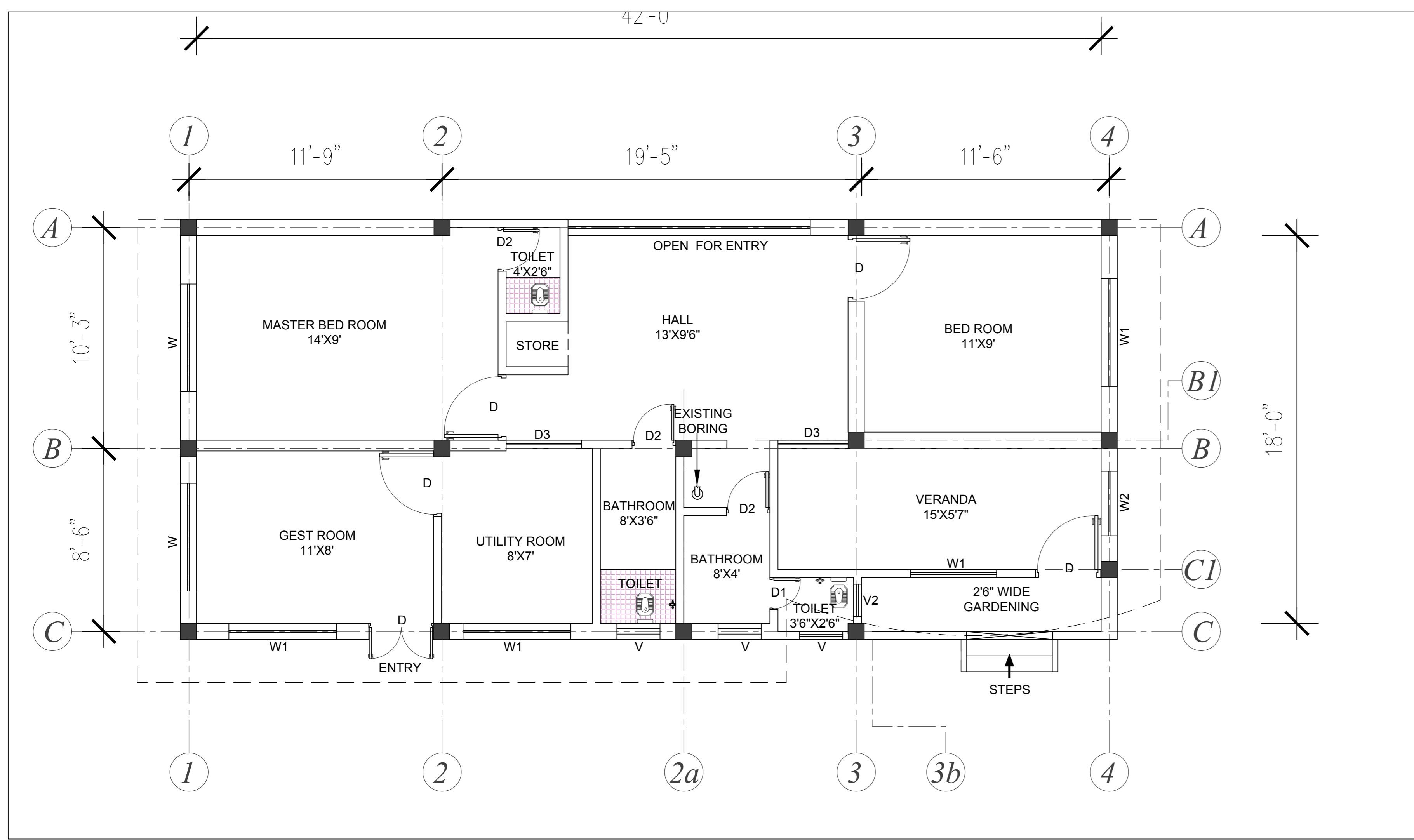
GROUND FLOOR PLAN-1
