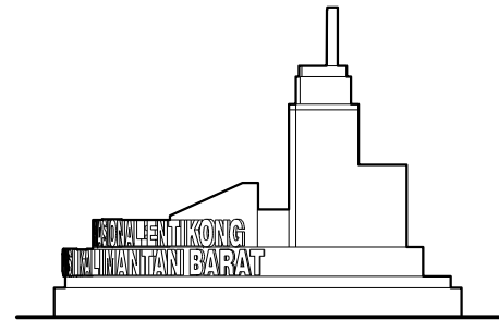
TAMPAK SAMPI NG TUGU GARUDA SKALA 1 : 50
