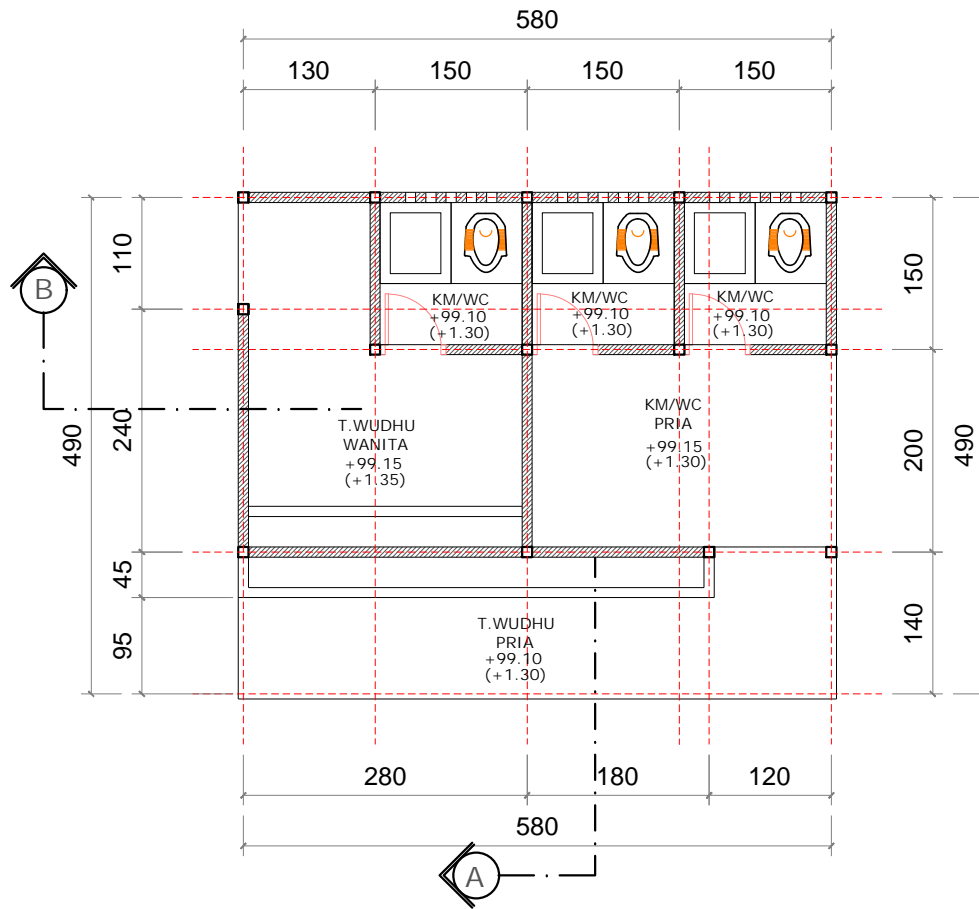
DENAH T.WUDHU skala 1:50
