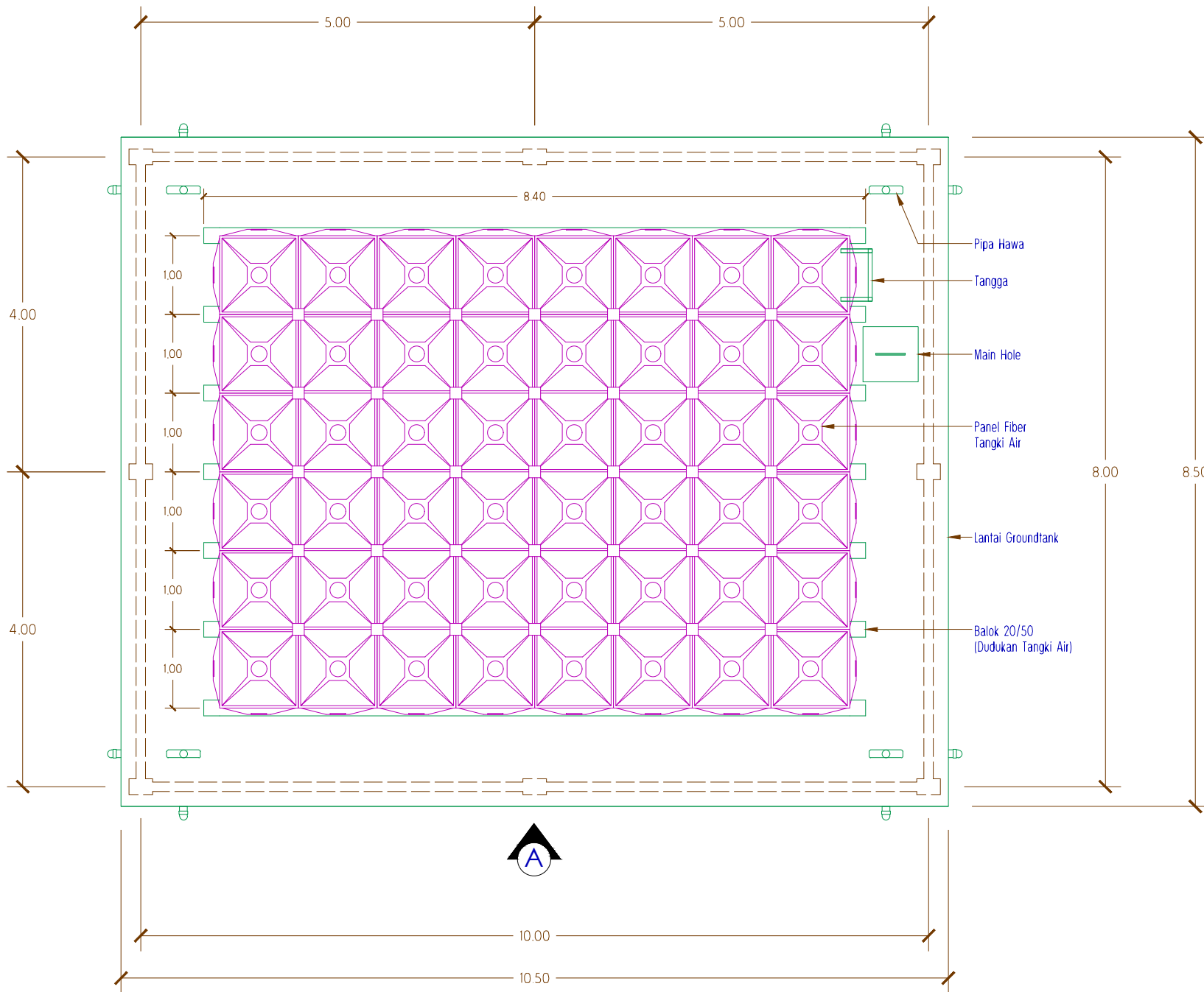
DENAH GROUNDTANK SKALA 1:50
