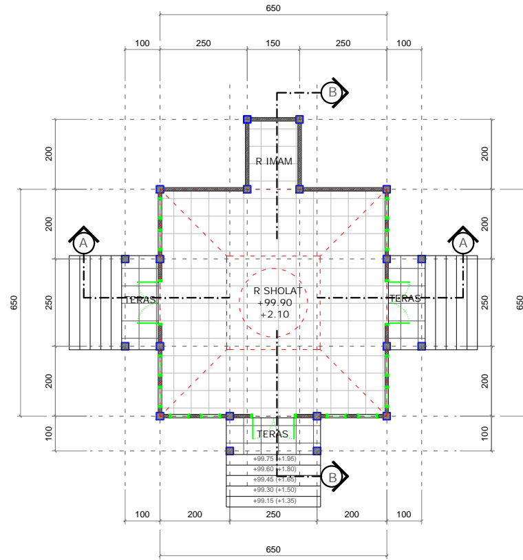
DENAH MUSHOLLA skala 1:100
