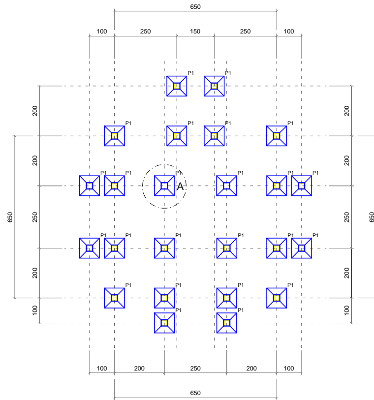
DENAH RECANAN PONDASI MUSHOLLA skala 1:100
