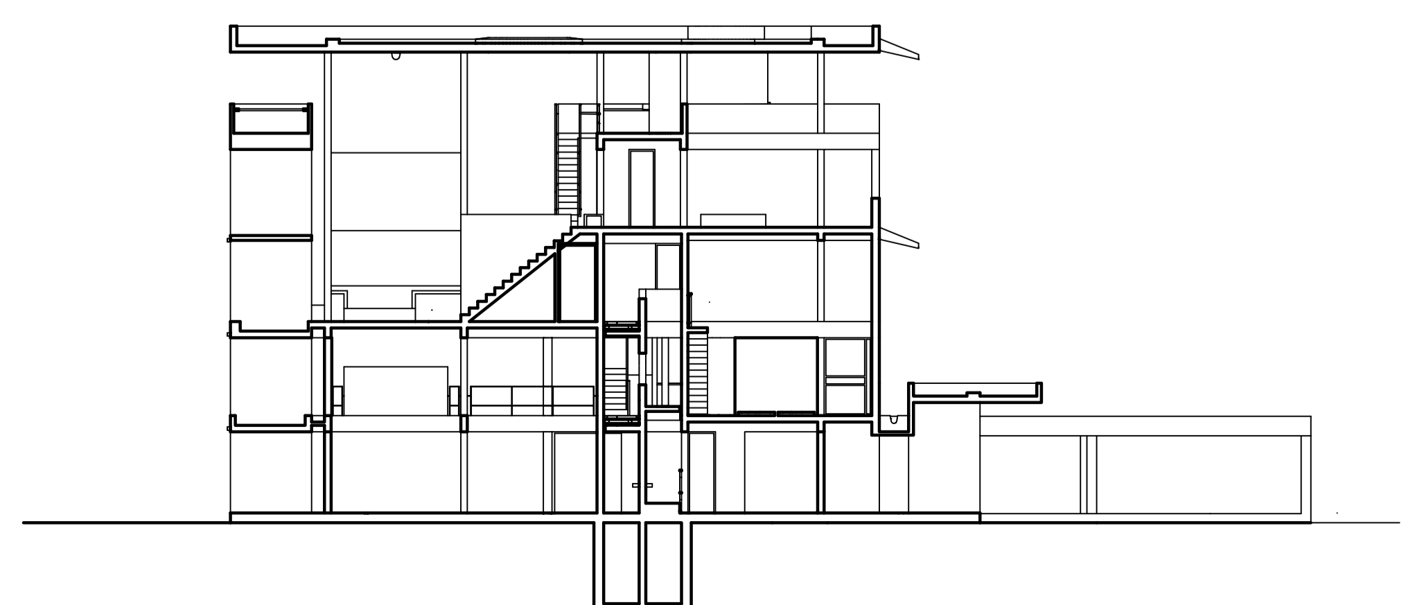
SECTION BB'
