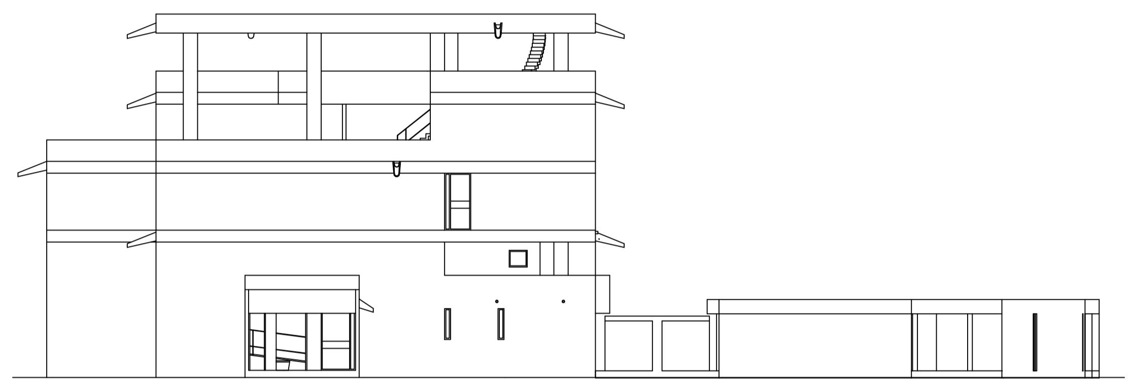
WEST SOUTH ELEVATION
