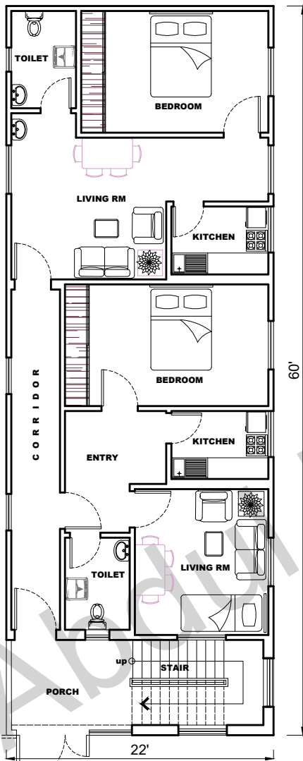
GF PLAN SCALE 1:100
