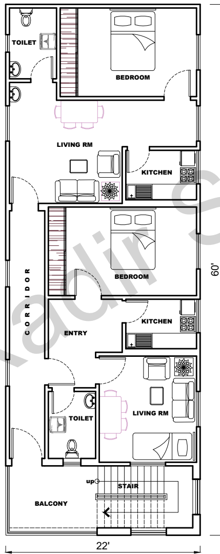
FF PLAN SCALE 1:100
