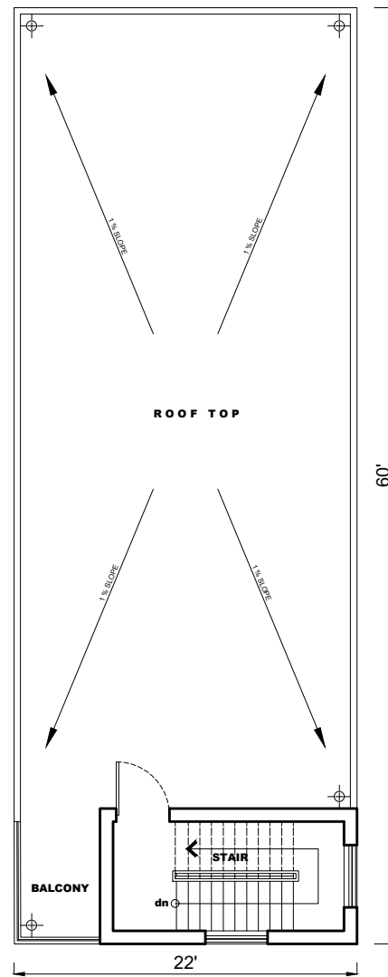
RF PLAN SCALE 1:100
