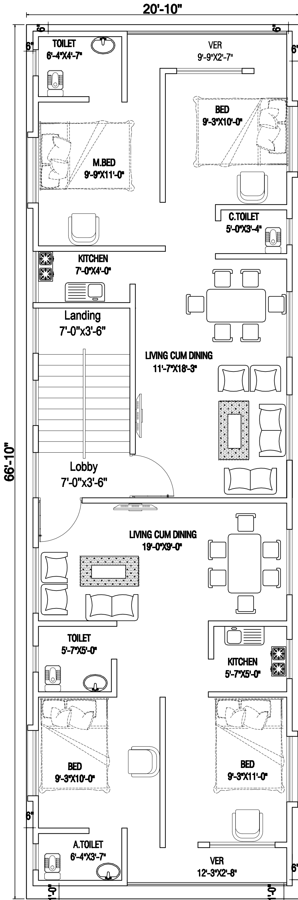
TYPICAL FLOOR PLAN
