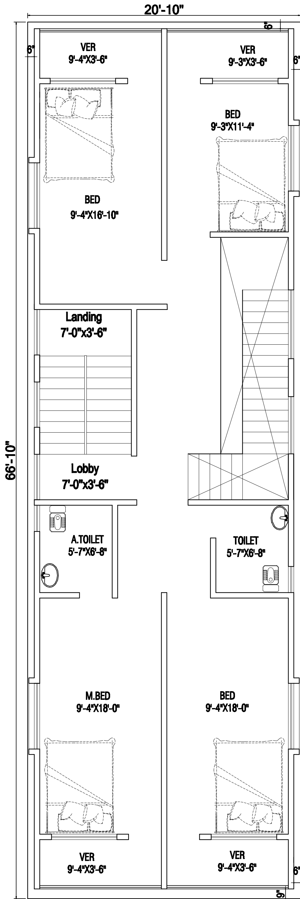
2ND FLOOR FURNITURE PLAN
