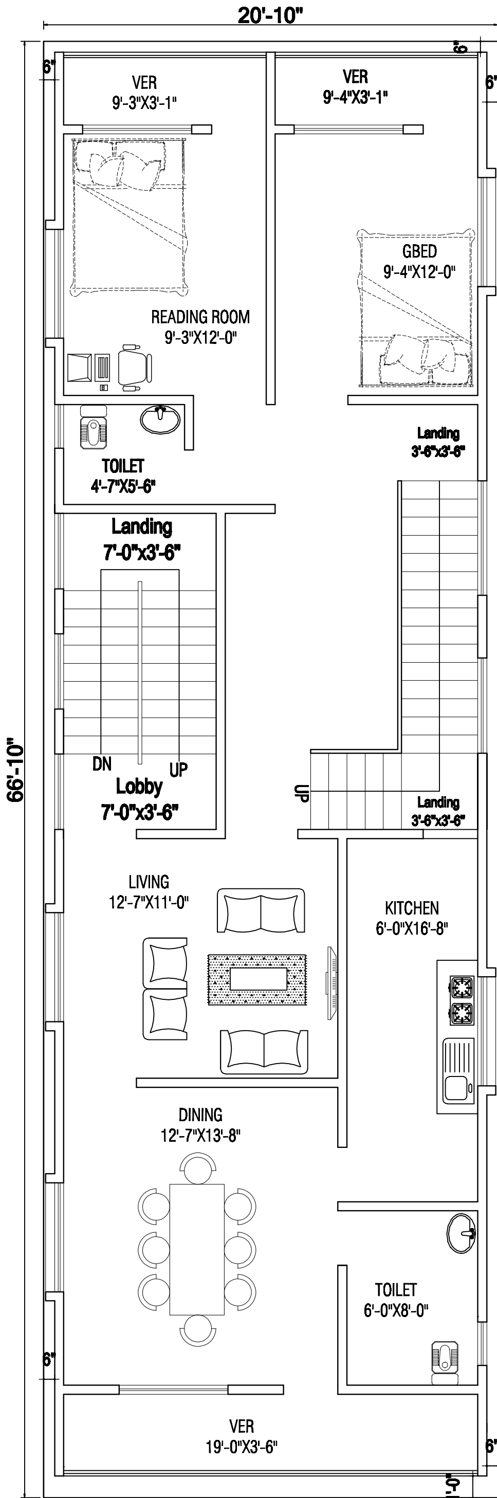
1ST FLOOR FURNITURE PLAN
