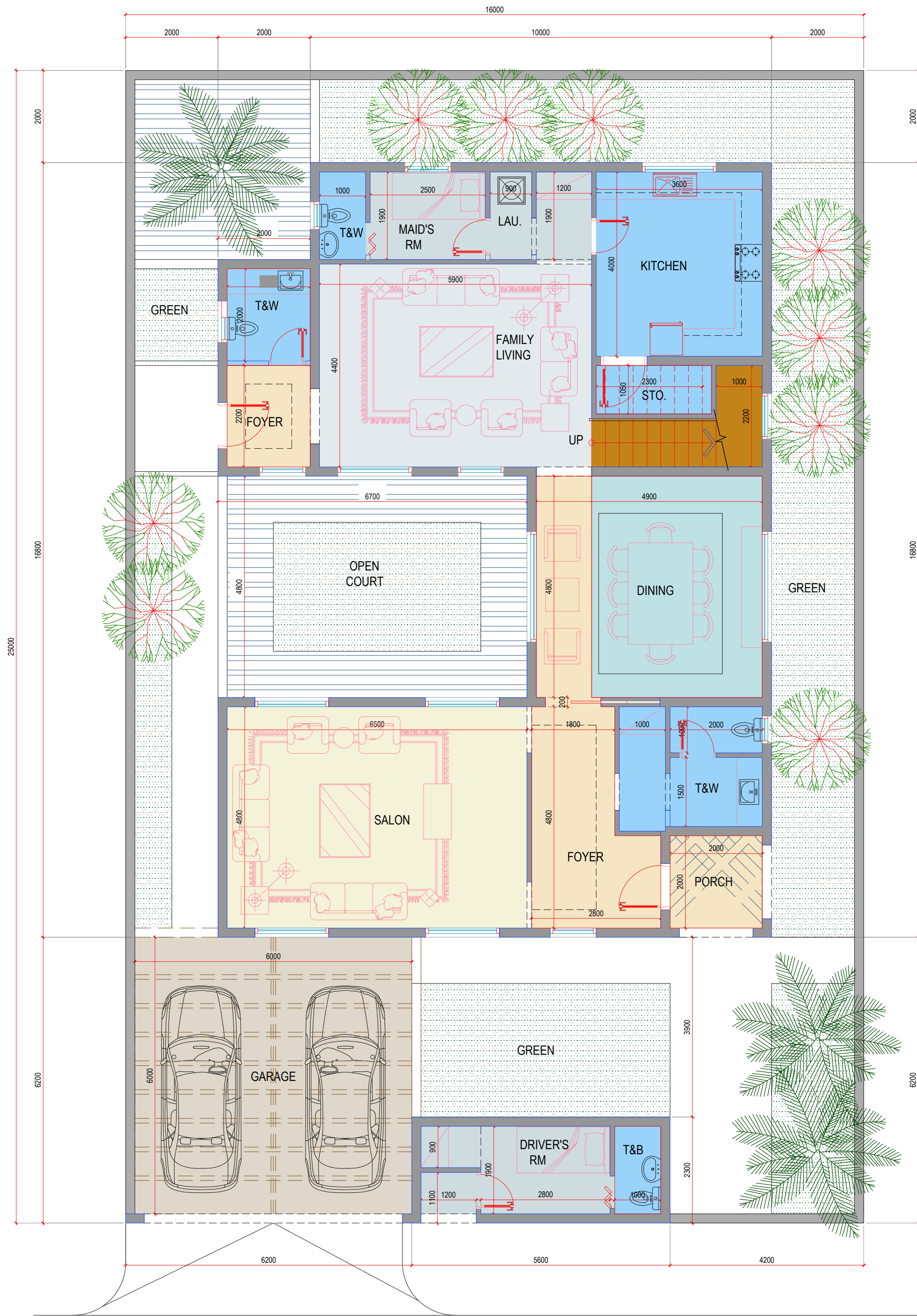
A AR-C1 GROUND FLOOR PLAN SCALE= 1:100M
