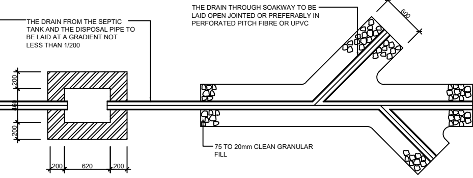
DISTRIBUTION CHAMBER
