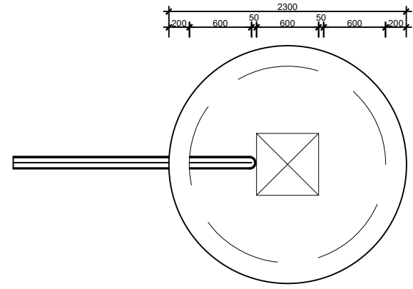
DISTRIBUTION CHAMBER
