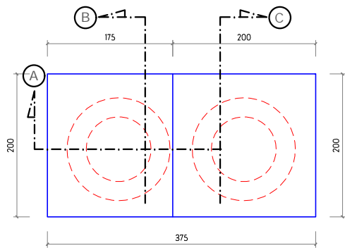
DENAH RENCANA TOWER AIR SKALA 1:50
