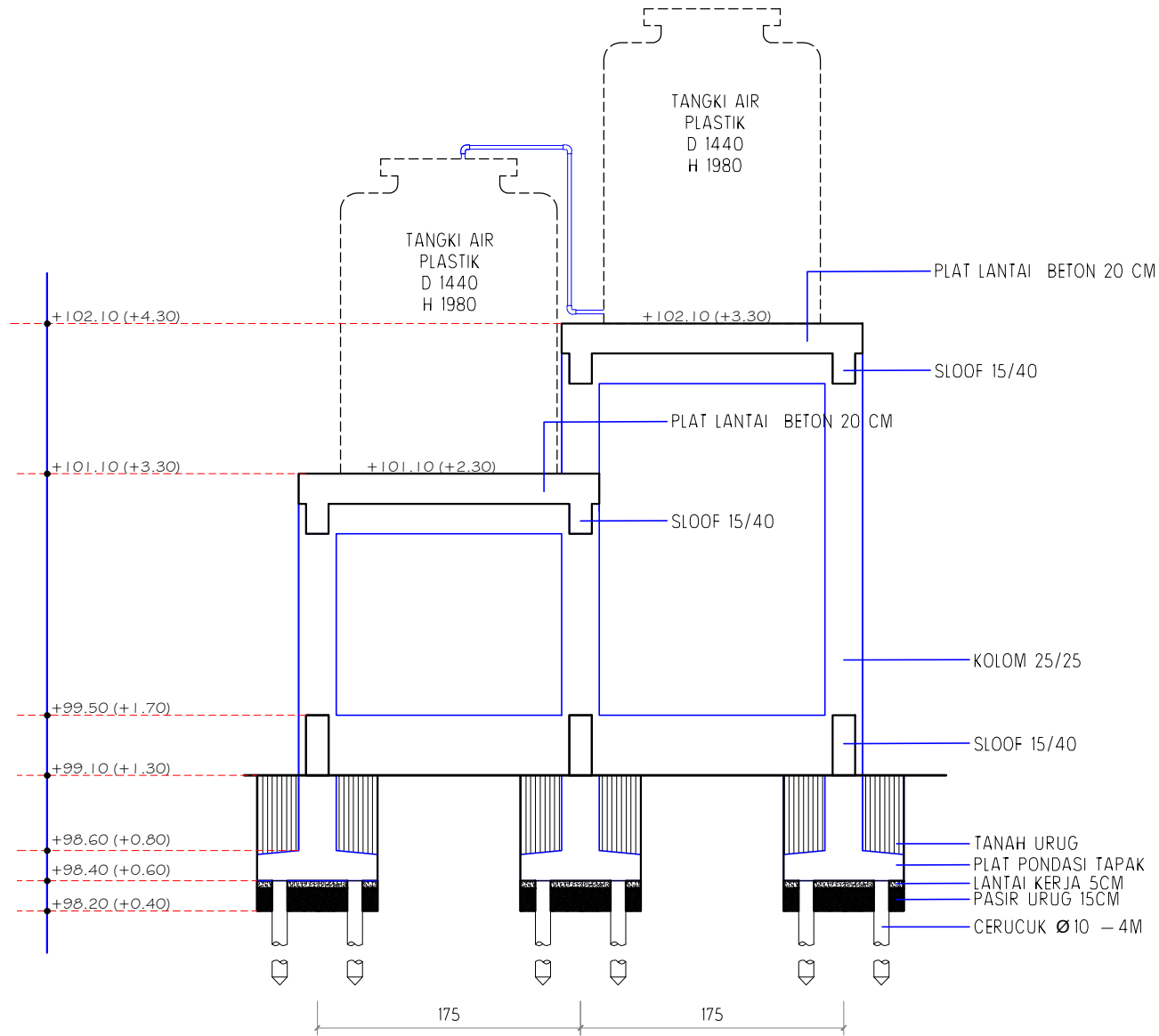
POTONGAN — A TOWER AIR SKALA 1:30
